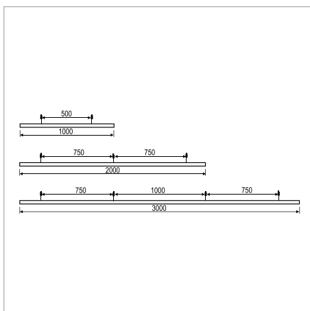
mounting holes
