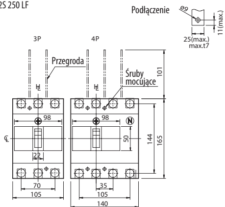
EB2S 250 LF
