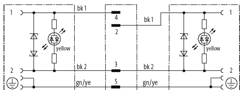
Valve plug 1
