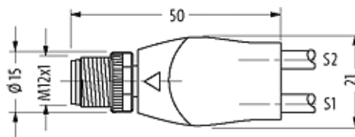
Valve plug 1
