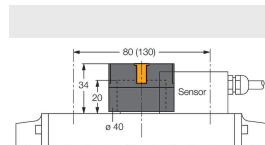
BTS-DSU35-EBE3 6901070
