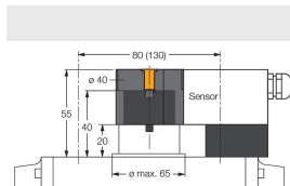
BTS-DSU35-Z02 6900230
