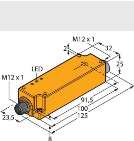
IMC-DI-22EX-PNO/24VDC 7560003
