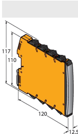
IMX12-DI01-2S-2T-0/7580020 24VDC
