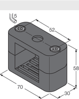
BSS-CP40 6901318
