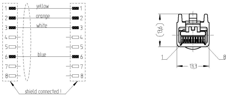
Contact Configuration
