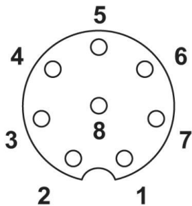
Pin assignment
