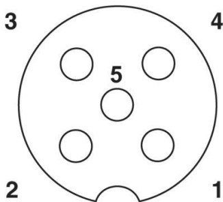
Wiring diagram
