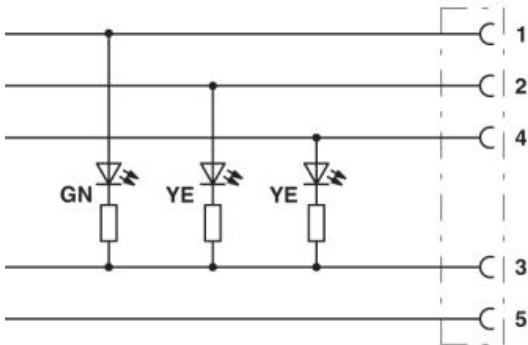
Wiring diagram
