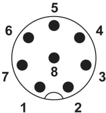
Pin assignment
