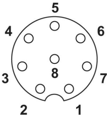
Pin assignment
