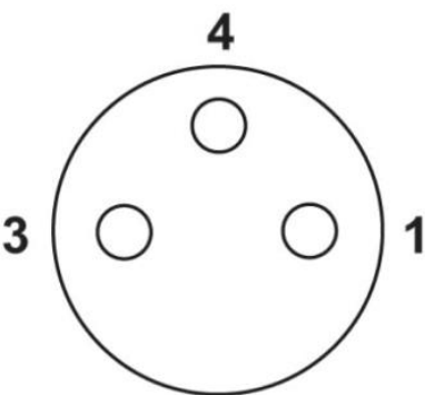
Wiring diagram
