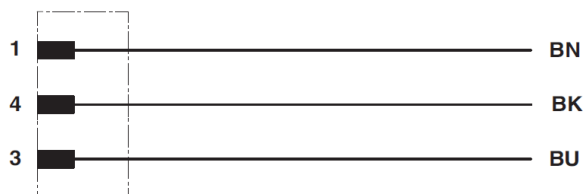
Pin assignment M12 plug
