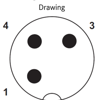
Pin assignment M12-plug, 3 pol, A-coding
