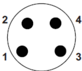
Pin assignment M8-plug, 4-pol, A-coding
