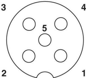
Pin assignment
