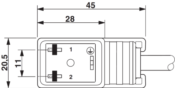
valve plug, design BI
