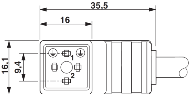
Valve plug, design CI
