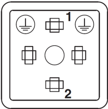
Pin assignment valve plug, design CI
