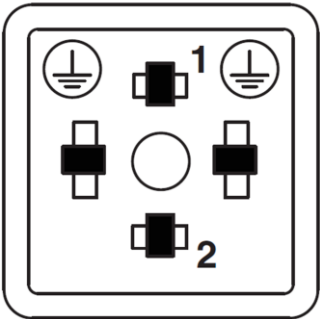
Pin assignment valve plug, design CI
