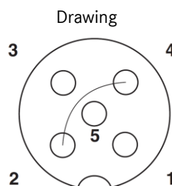
Pin assignment M12-jack, 3 pol, bridged, with PE, A-coding
