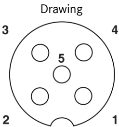
Pin assignment M12-jack, 5 pol, A-coding
