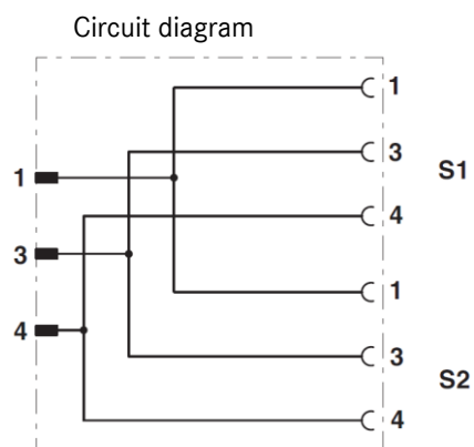
Pin assignment M8 Y-distributor
