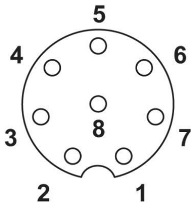
Pin assignment
