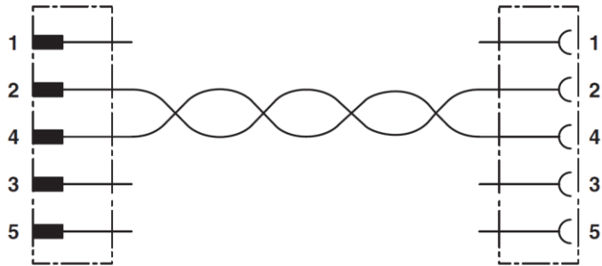
Circuit diagram
