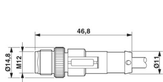
Dimensioned drawing, M12 plug
