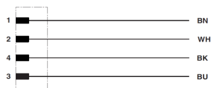
Contact assignment M12-plug and M12-jack
