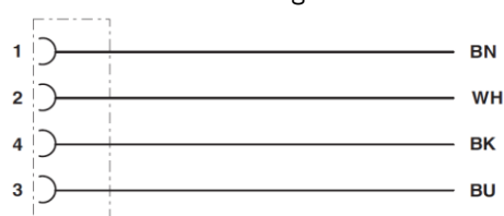
Contact assignment M12-plug and M12-jack
