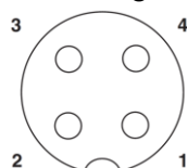
Pin assignment M12-jack, 4-pos., A-coding
