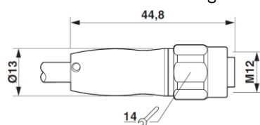
Dimensional drawing
