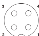
Pin assignment M12-jack, 4-pos., A-coding
