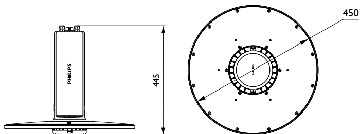
CoreLine High-bay BY120P/BY121P
