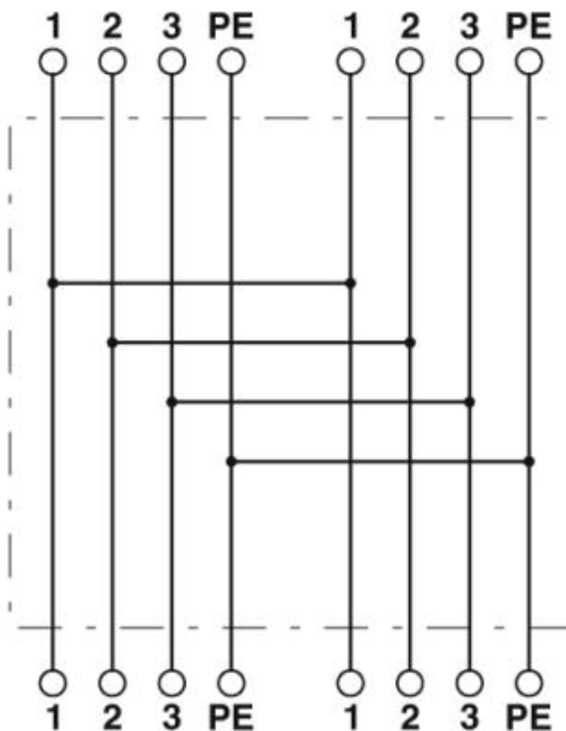
Circuit diagram
