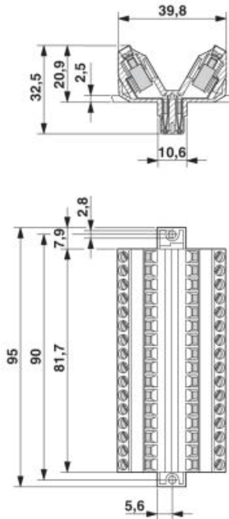
Dimensional drawing
