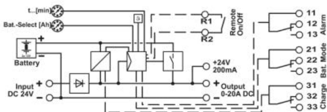
Block diagram
