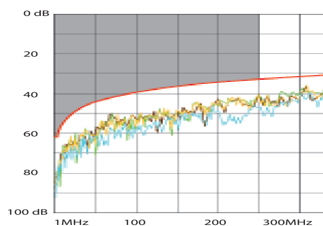
PS NEXT (Power Sum NEXT)
