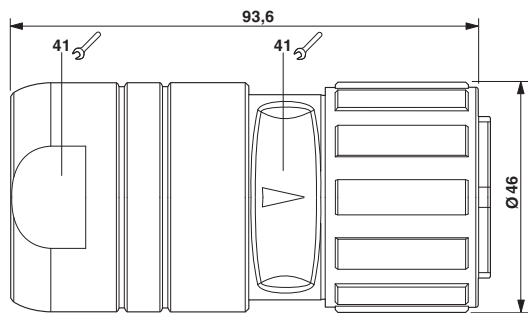
Dimensional drawing
