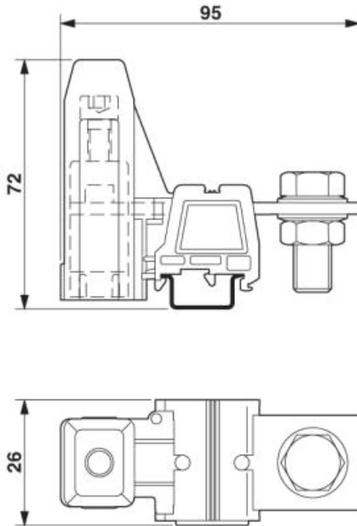
Dimensional drawing
