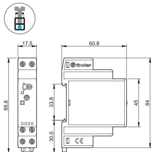
15.10 Screw terminal
