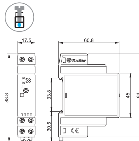
15.11 Screw terminal
