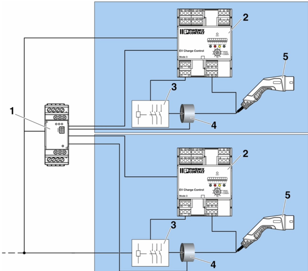
Connection diagram
