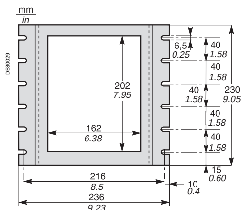
Support de montage AMT840
