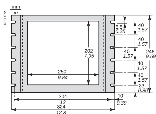
Support de montage AMT880.
