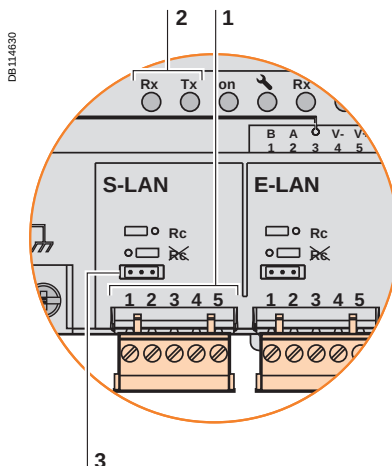
Port S-LAN (ACE969TP-2)
