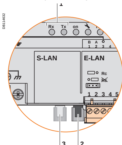
Port S-LAN (ACE969FO-2)
