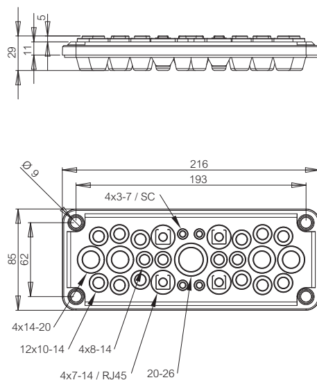
FIBOX FM C-25F
