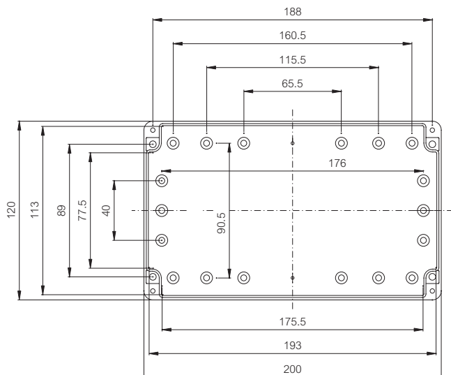
EURONORD PC/ABS 200x120x75-90
