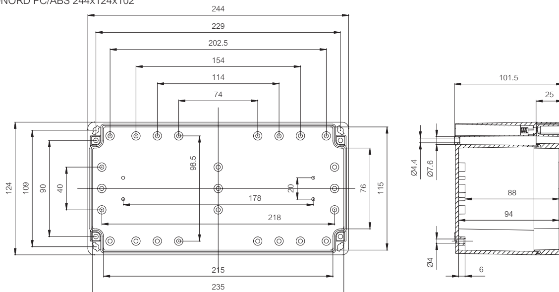
EURONORD PC/ABS 244x124x102
