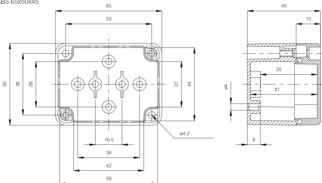
EURONORD PC/ABS 65x50x45
