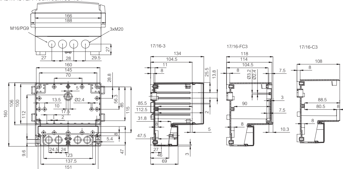
CARDMASTER 166x160x108-134
