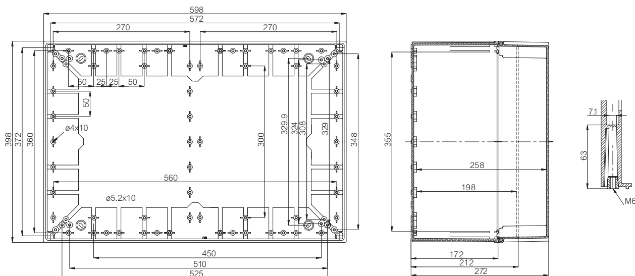
QUICK 600x400x210-270
