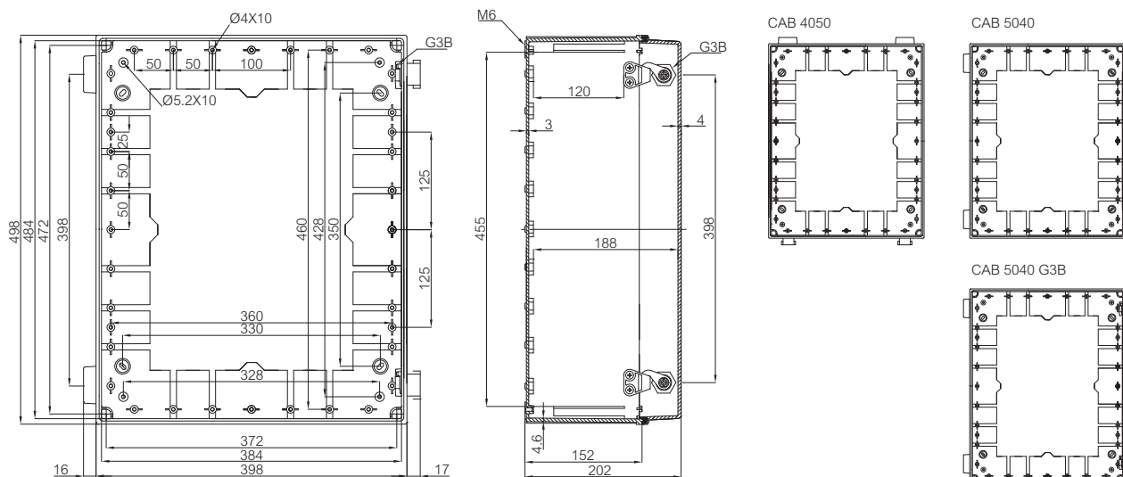
CAB 500x400x200
