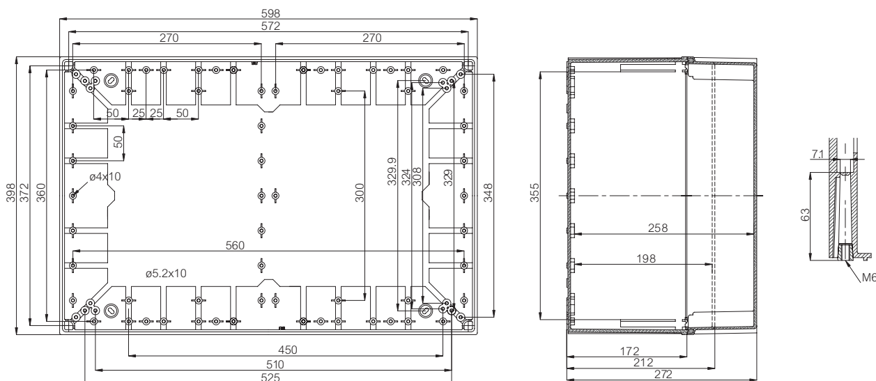
QUICK 600x400x210-270
