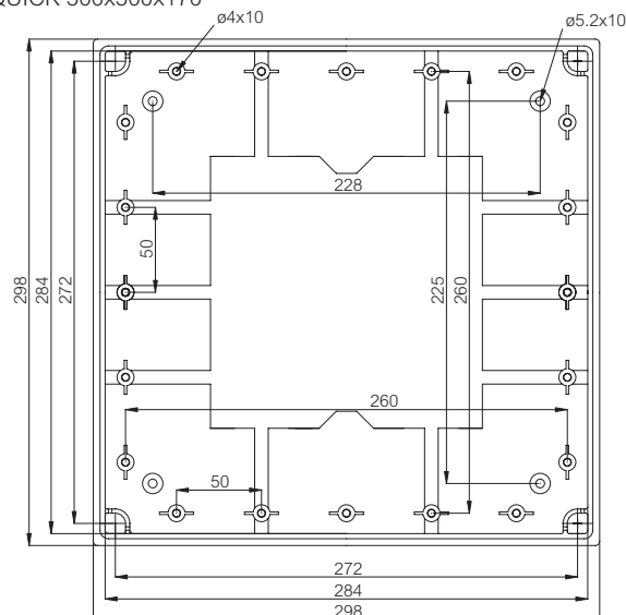
QUICK 300x300x170
