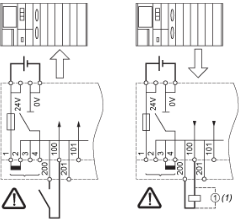
(1) Inductive load
