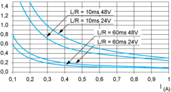
DC13 curves
