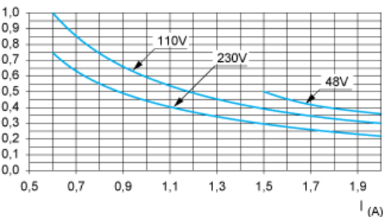
AC15 curves
