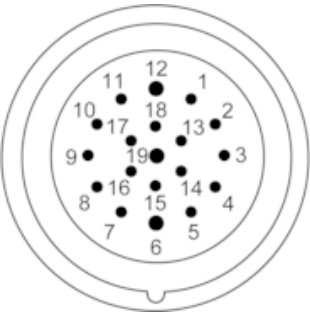
M23 Connector
