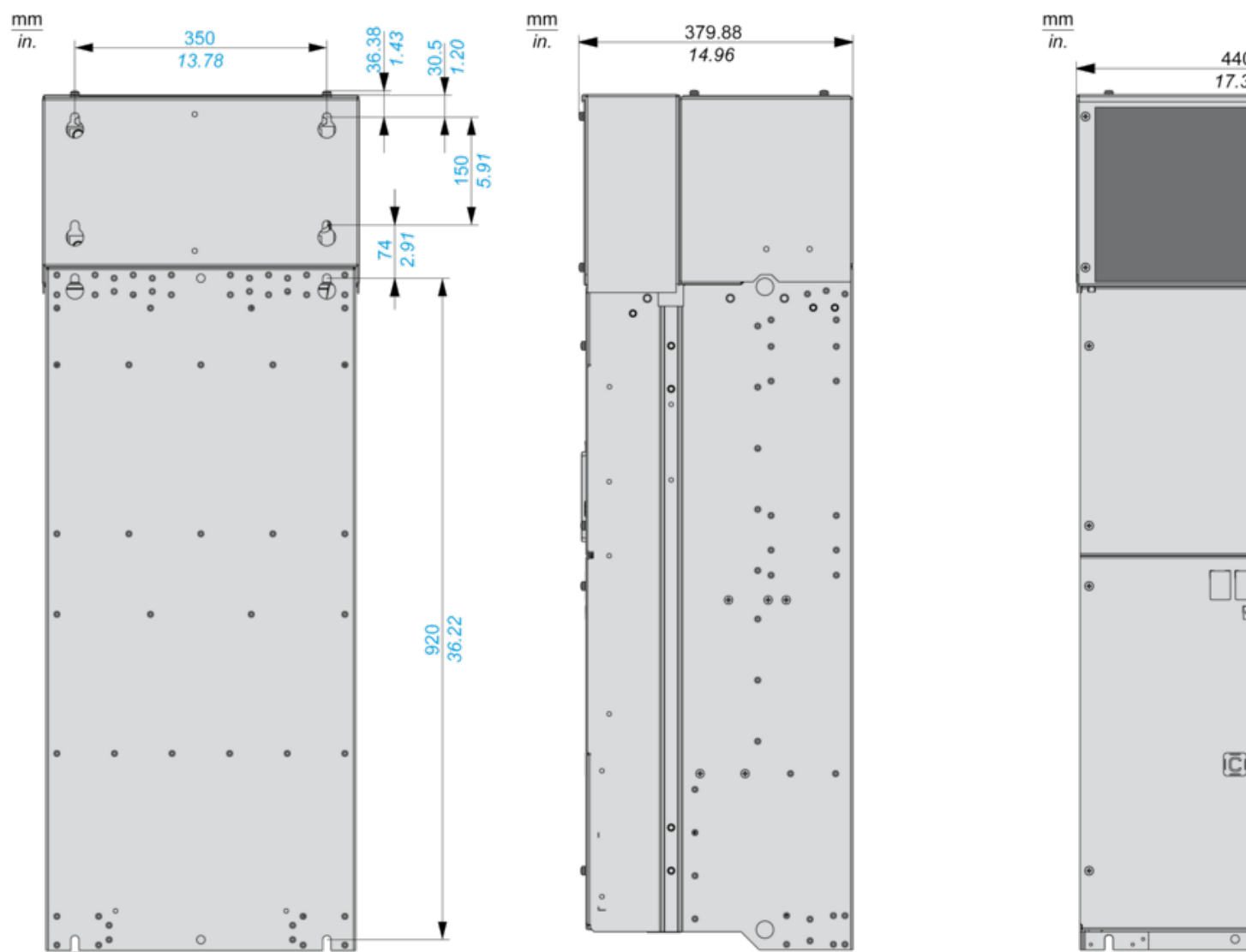
Rear, Right and Front View
