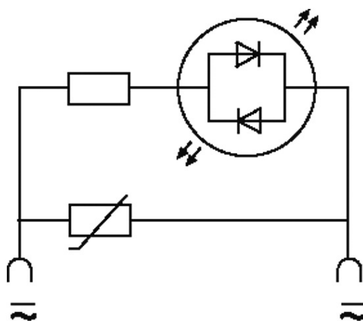
LED + VDR
