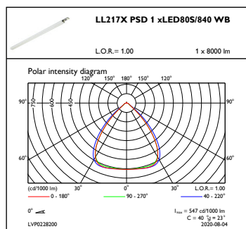
OFPC1_LL217XPSD1xLED80S840WB
