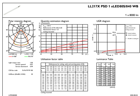
IFGU1_LL217XPSD1xLED80S840WB
